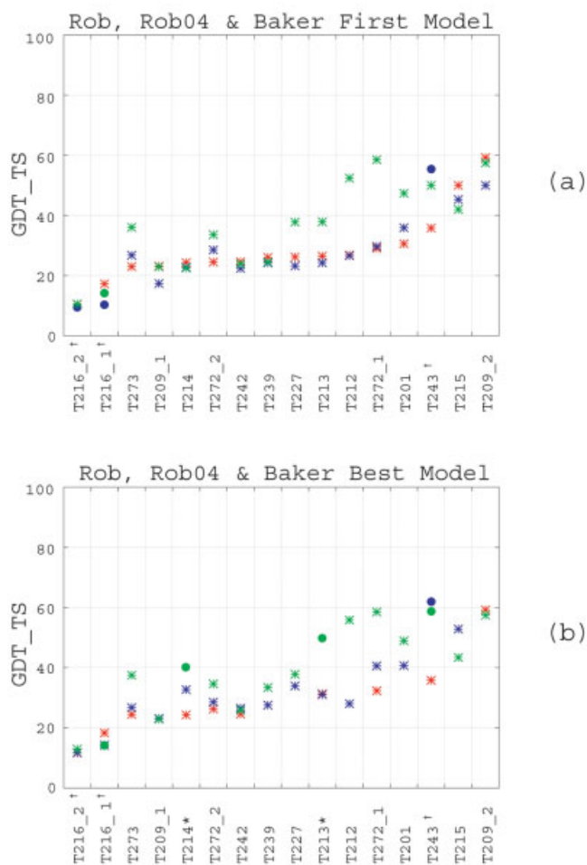
Fig. 3. Target-specific model quality for Robetta, Robetta_04, and Baker human group in the de novo regime. a : The absolute GDT_TS score of the First model of Robetta (in red), Robetta_04 (in blue), and the Baker human group (in green). De novo models are indicated with an asterisk, and template-based models with a circle. b : The absolute GDT_TS score of the Best model of Robetta, Robetta_04, and the Baker human group, with colors and point types as before. *: the best Baker human models for targets T0213 and T0214 were template-based models using a parent suggested by Alexey Murzin. †: the 3D-Jury confidence changed between the release of the target sequence and the due date of each target for targets T0216 and T0243, leading these targets to be considered “twilight-zone” targets and modeled by both template-based and de novo protocols by Robetta_04, and using a template-based approach by the Baker human group.
